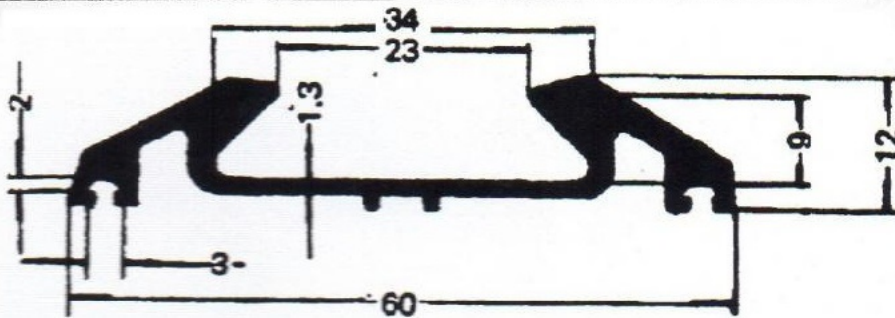
B-E2506 (554 gr/mt)
